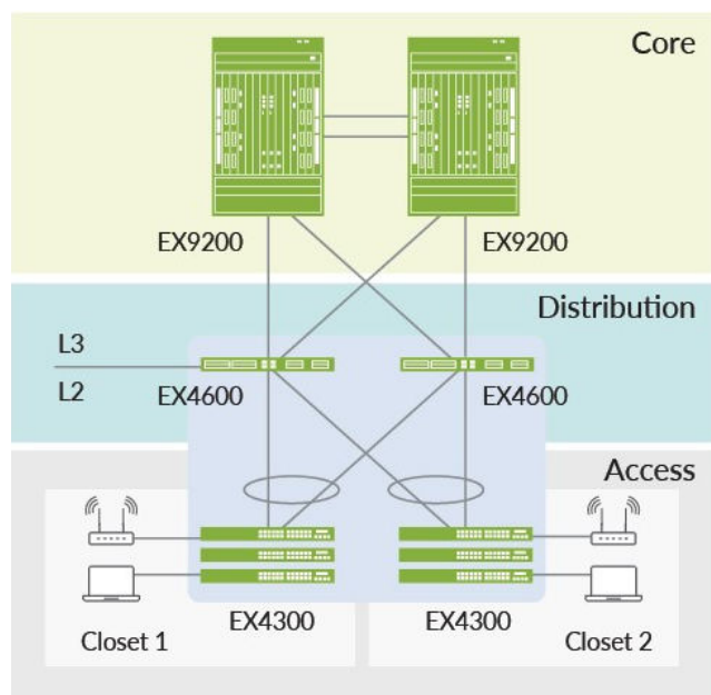
Figure 5: Mixed Virtual Chassis configuration with EX4600 and EX4300 switches.
